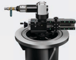
FI700 Flange Facing Machine
