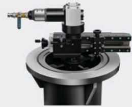
FI700 Flange Facing Machine
