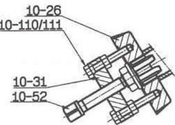
MILLING CUTTER EXTRACTION TOOL
